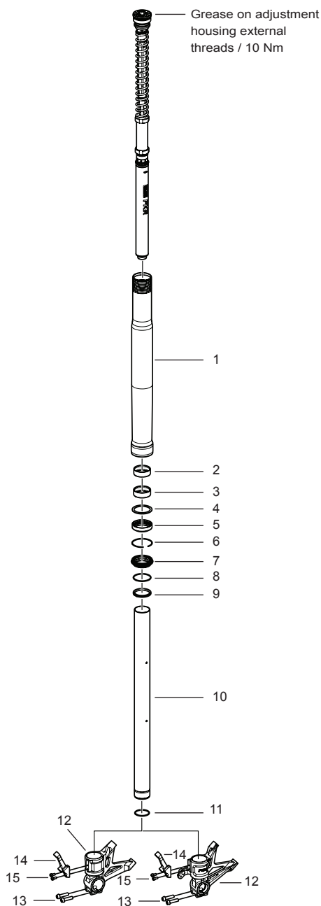
Figure 5 - External components
