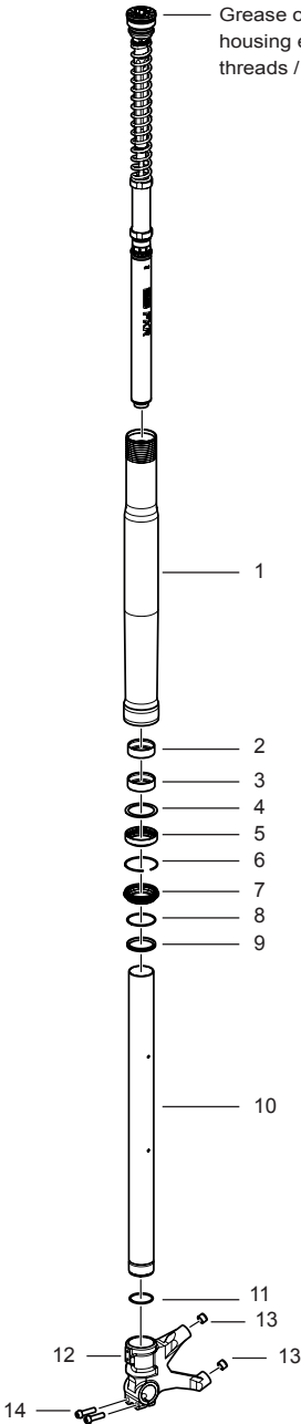
Figure 5 - External components
