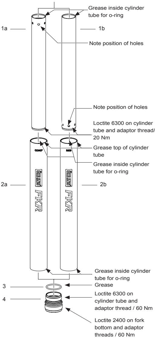
Figure 4 - Cylinder tube assembly
