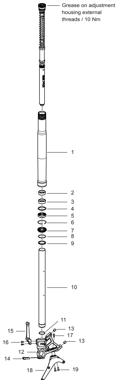
Figure 5 - External components
