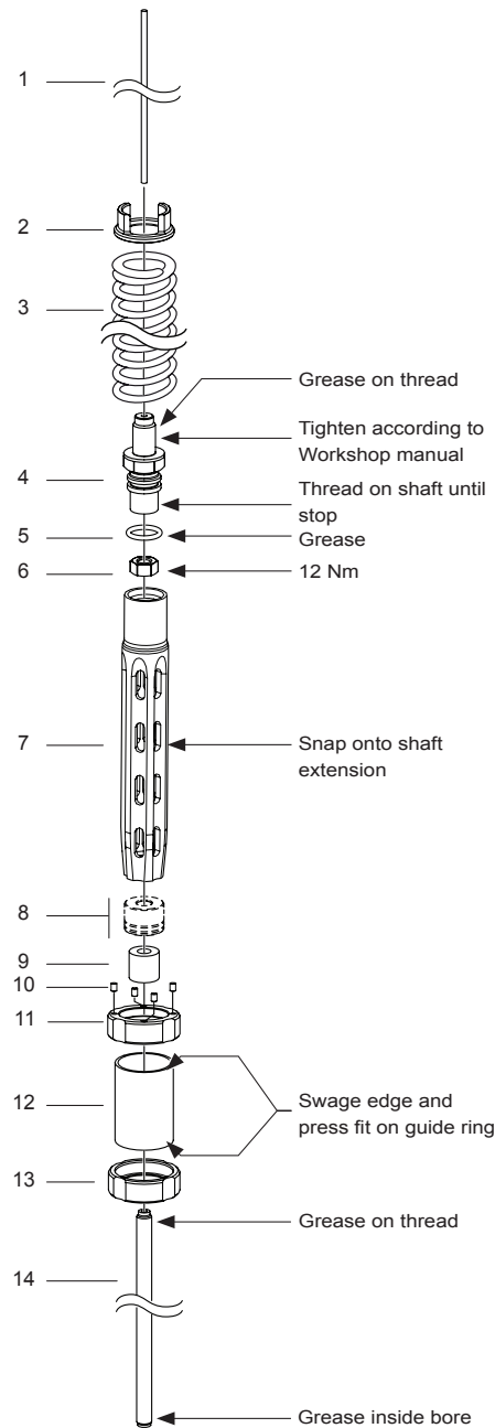
Figure 2 - Shaft assembly
